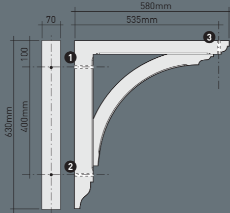
GB03 70 x 630 x 580mm 2 3 / 4 " x 24 13 / 16 " x 22 7 / 8 " - structural max. 75kg* - white wood grain finish
